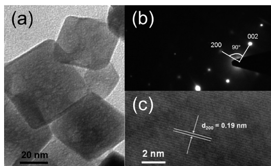
Figure 3. (a) TEM image of cubic \text{TiO}_2 NCs obtained in 12 h showing their sharp edges, (b) SAED spots of cubic \text{TiO}_2 NCs showing the diffracted planes and angle between them, and (c) the corresponding lattice fringe matching the distance between (200) planes of bulk \text{TiO}_2 crystals.
