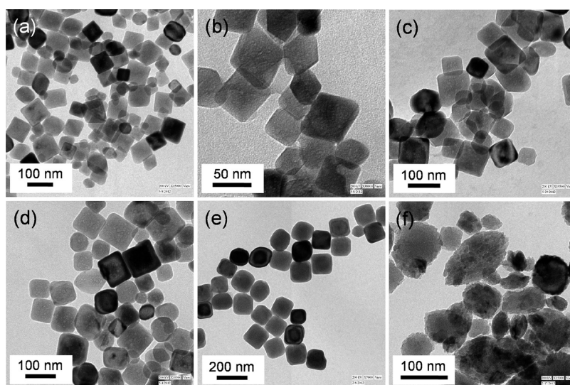
Figure 2. TEM images of \text{TiO}_2 NCs synthesized by hydrothermal process at 225^\circ\text{C} with a reaction duration of (a, b) 12 h, (c) 24 h, (d) 36 h, (e) 48 h, and (f) 72 h.
